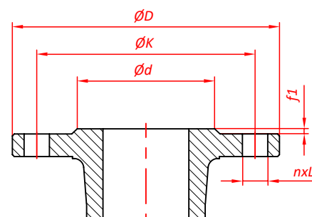
RF FLANGE
